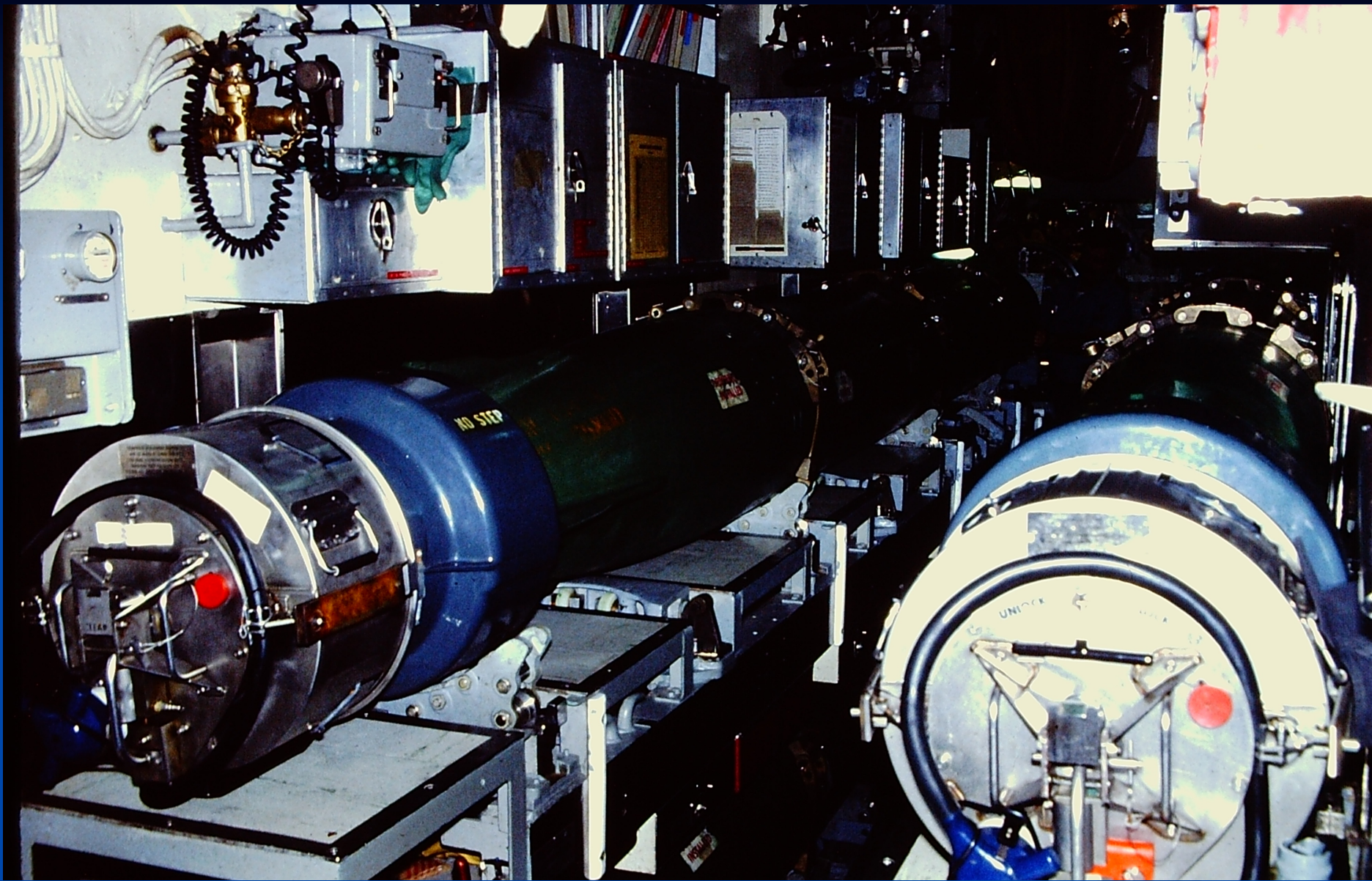
TORPEDO ROOM
